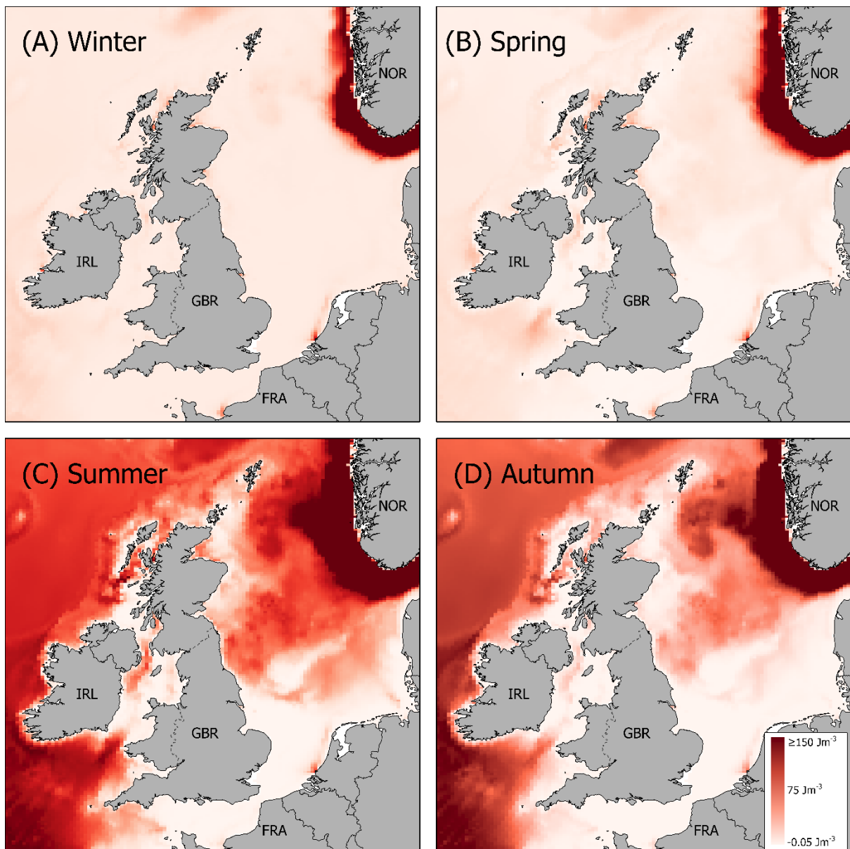
Figure 6. Vertical stratification ( J/m^3 ). The vertical stratification raster (potential energy anomaly) raster was obtained from the Ensemble Statistics dataset calculated from the Northwest Shelf Perturbed Parameter Ensemble (NWPPE). The NWPPE provided seasonal means for PEA from 2000 to 2019 at 7 \times 7 km horizontal resolution. Countries labelled with ISO 3166 three-character codes.
