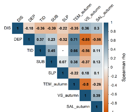
Figure 3. Seasonal environmental correlation matrices. Correlation matrices describing median rho from 1000 simulations of 250 random locations to sample spatially coincident environmental variables. Median rho shown for significant relationships ( p < 0.05 ; with Fishers' adjustment). Seabed bottom temperature (TEM), salinity (SAL), vertical stratification (VS), tidal speed (TID), seabed depth (DEP), seabed slope (SLP), distance from shore (DIS), seabed substrate (SUB).
